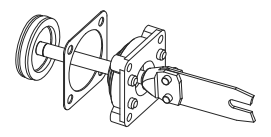
NO.202 Assembly 47,48,49
